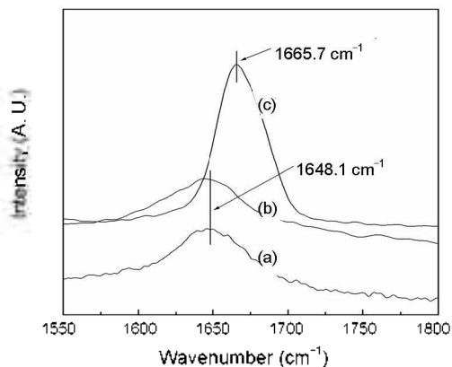
Fig. 5. Raman spectra of (a) 0.1 M/10 wt%-PVP/Ag composites solution, (b) 10 wt% PVP in H 2 O and (c) solid PVP.
