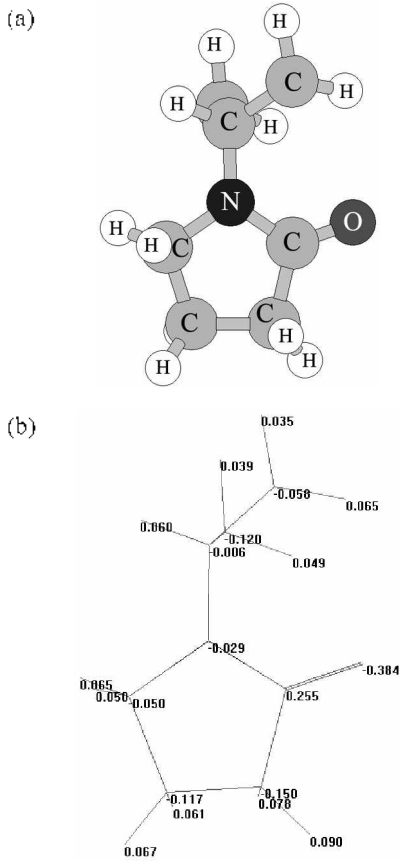
Fig. 2. Chemical structure and net charge of PVP monomer: (a) three dimension structure (b) net charge. (calculated from HyperChem 6.0 program)
