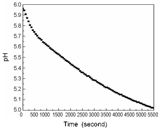
Fig. 7. Time evolution of pH after addition of 0.1 M \text{AgNO}_3 on to 10 wt% PVP.
