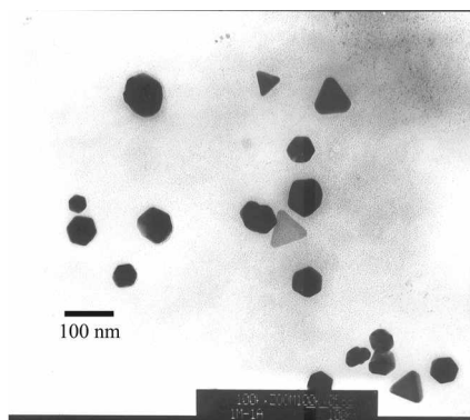
Fig. 4. TEM image of silver nanoparticles for 0.1 M/10 wt%-PVP/Ag composites solution.
