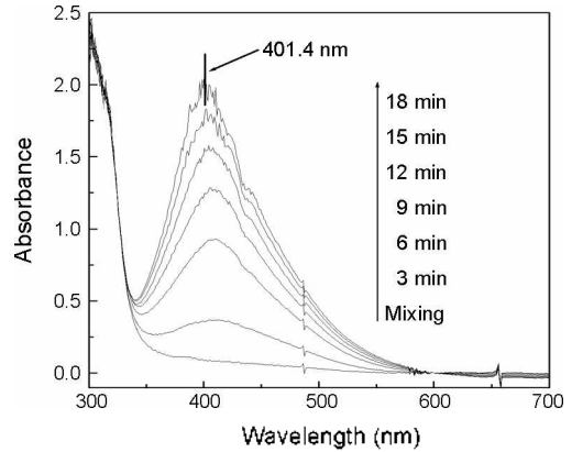
Fig. 3. Time evolution of UV-VIS spectra after addition of 0.1 M AgNO 3 on to 10 wt% PVP.
