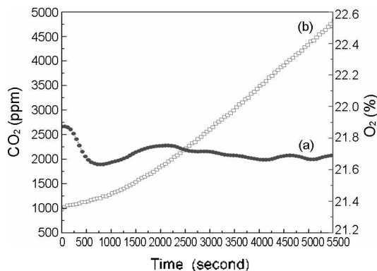
Fig. 6. Time evolution for concentration of (a) O 2 and (b) CO 2 after addition of 0.1 M AgNO 3 on to 10 wt% PVP.
