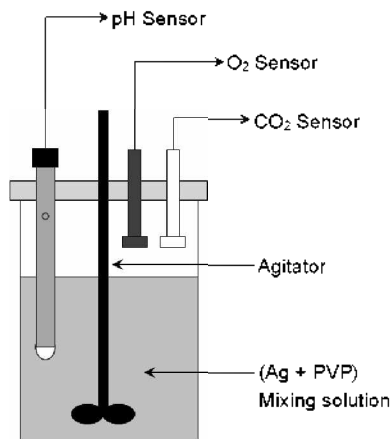
Fig. 1. The diagram of PVP/Ag composites analysis system.
