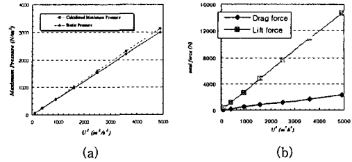
Fig. 3 (a) Calculated maximum pressure and theoretical static pressure for various speeds (b) Drag and lift force for various speeds
