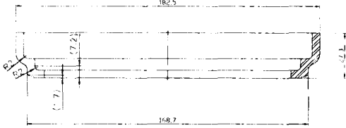
Fig. 1 Drum shape part for auto transmission: drum-lock-up
