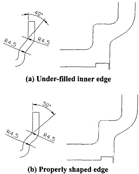
(a) Under-filled inner edge (b) Properly shaped edge Fig. 6 Effect of drawing inclination on the edge filling
