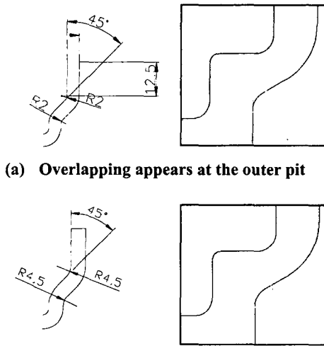
(a) Overlapping appears at the outer pit (b) Overlapping is resolved by larger corner radius Fig. 5 Effect of fillet radius of drawn work piece
