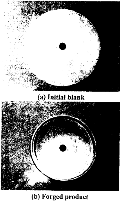
Fig. 7 Drum-lock-up produced by combination of deep drawing and forging
