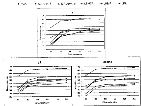
Figure 4. The recognition performance of PCA, ICA1, ICA2, LNMf, LFA and LS-ICA methods for the AR facial databases.
