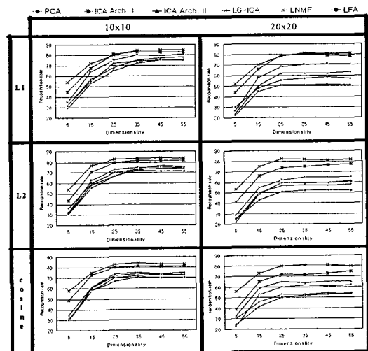
Figure 5. Recognition performance versus the size (in 10x10, 20x20) of occluding patches for PCA, ICA1, ICA2, LNMf, LFA, and the proposed LS-ICA method for the AT&T database.
