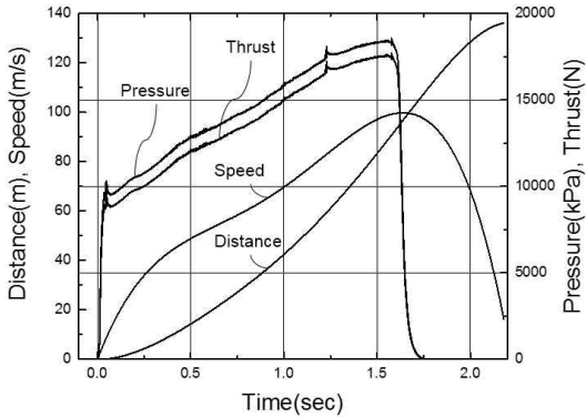
Fig. 3. Measured combustor pressure, thrust, distance and speed of the underwater vehicle
