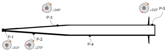
Fig. 4 Positions of pressure sensors installed on the vehicle tested
