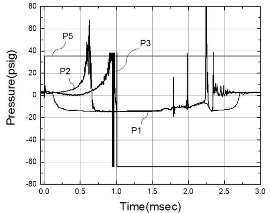
Fig. 5. Pressures measured on the vehicle surface
