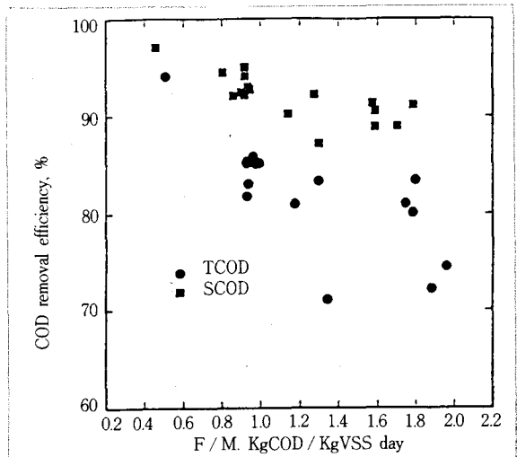
그림 3. Relationship between COD removal efficiency and F / M ratio.
