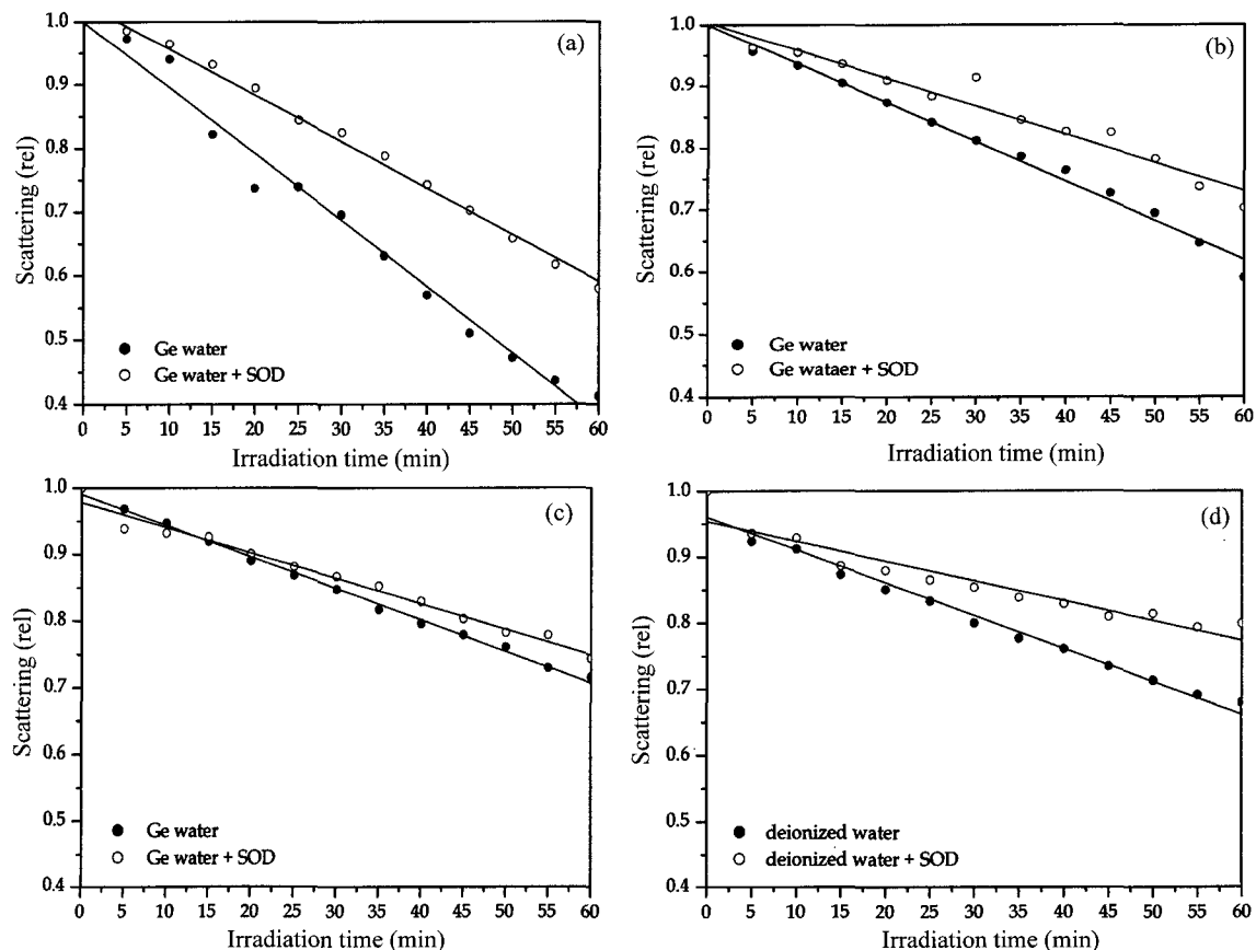
Figure 2. Photodissociation rate of the liposomes with and without superoxide dismutase in different water: (a) Ge water - 0.24 \mu\text{g}/\text{ml} \text{Ge}^{4+} ion, (b) Ge water - 0.12 \mu\text{g}/\text{ml} \text{Ge}^{4+} ion, (c) Ge water - 0.073 \mu\text{g}/\text{ml} \text{Ge}^{4+} ion, (d) deionized water.
