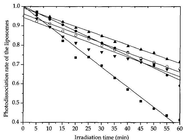
Figure 1. Photodissociation rate of the liposomes as a function of \geq 320 \text{ nm} irradiation in different water: (■) Ge water - 0.24 \mu\text{g/ml} \text{Ge}^{4+} ion, (●) Ge water - 0.12 \mu\text{g/ml} \text{Ge}^{4+} ion, (▼) plain mineral water, (○) deionized water, (▲) Ge water - 0.073 \mu\text{g/ml} \text{Ge}^{4+} ion.
