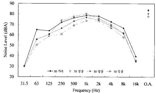
그림 6 Pass-by noise spectra of typical heavy vehicle(15t dump truck)
