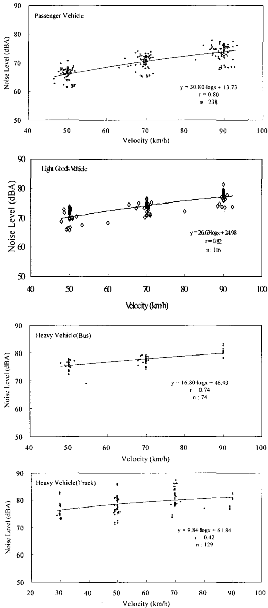
그림 2 Relationship between steady state speed and noise level
