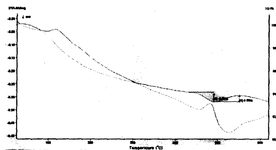
Fig. 1 Thermograms of cement-fly ash paste at 28 day
