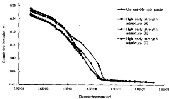
Fig. 4 Pore structure of cement-fly ash paste containing high early strength admixtures at 1 day
