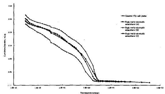
Fig. 5 Pore structure of cement-fly ash paste containing high early strength admixtures at 7 day
