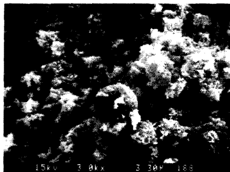
d) Cement-fly ash paste with high early strength admixture C (3, 28 day)
