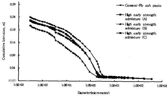
Fig. 6 Pore structure of cement-fly ash paste containing high early strength admixtures at 28 day
