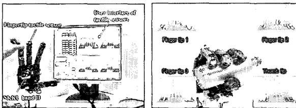
(a) SKKU hand II (b) Experiment of power grasping task
