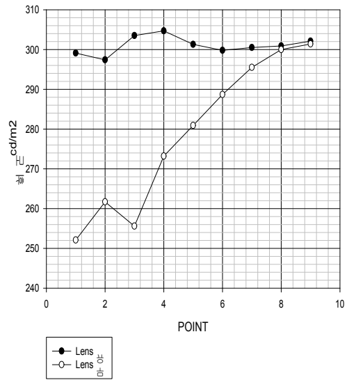
Figure 8: The characteristics of the brightness uniformity
