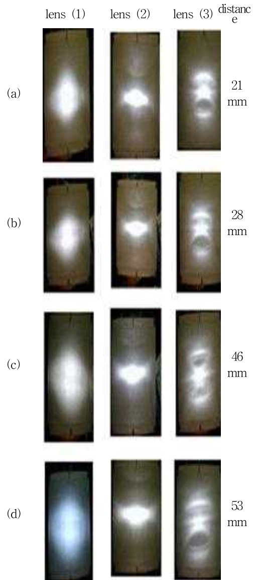
Figure 4: The light image of the different dimensions of the lenses
