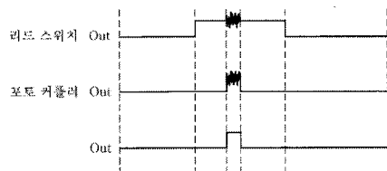
(a) Reed SW, Photocoupler, OUT Output
