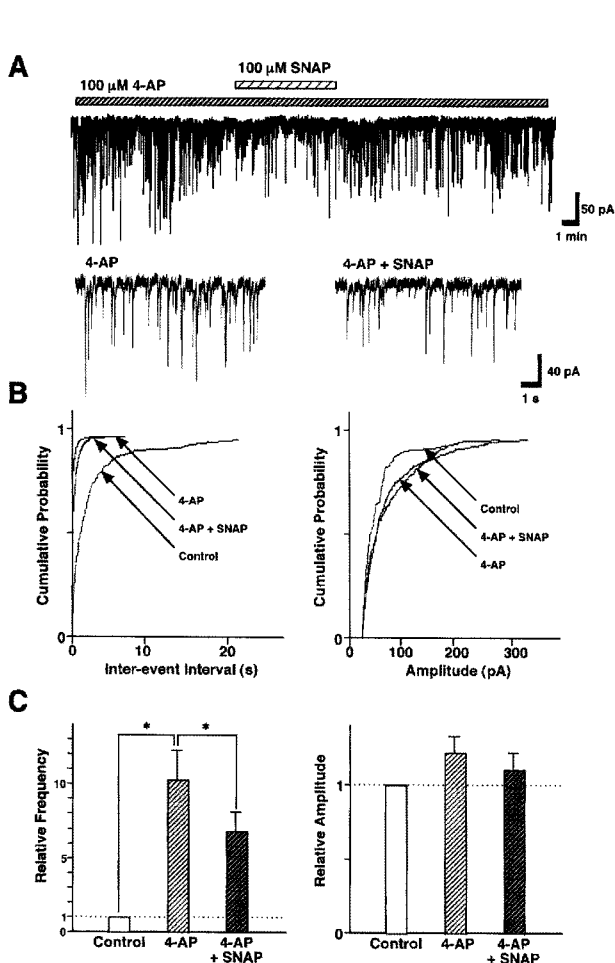
Fig. 5. Effect of the 4-aminopyridine on the SNAP-induced inhibition of GABAergic sIPSCs. (A) Representative recording traces of sIPSCs show the change in the SNAP effect in the presence of 100 \mu M 4-AP, a K^+ channel blocker. Insets represent typical traces with an expanded time scale. (B) Cumulative distributions for inter-event interval (left) and amplitude (right) of sIPSCs in the same neuron. p values indicate the results of K-S tests for frequency and amplitude. (C) All amplitudes and frequencies are normalized to the control sIPSCs. Each column is the mean of 9 neurons. Asterisks represent a statistically significant difference ( *p < 0.05 , paired two-tailed t -test).
