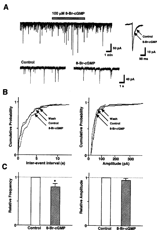
Fig. 3. SNAP-induced presynaptic inhibition of GABAergic sIPSCs is coupled to the cGMP-dependent signal transduction pathway. (A) A representative trace of sIPSCs recorded before, during, and after the application of 100 \mu M 8-Br-cGMP. Insets, represent typical traces with an expanded time scale (lower) and 8-Br-cGMP-induced changes in the rate of rise and decay time constant (upper). (B) Cumulative probability distributions for inter-event interval (left) and amplitude (right) of GABAergic sIPSCs recorded from the same neuron. p values indicate the results of K-S tests for frequency and amplitude. (C) Each column is the mean of 6 neurons. All frequencies and amplitudes are normalized to those of control sIPSCs. Asterisks represent a statistically significant difference ( *p < 0.05 , paired two-tailed t -test).
