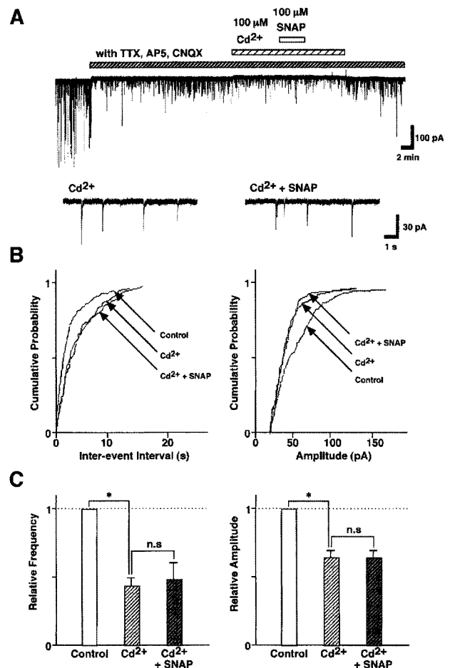
Fig. 6. SNAP-induced inhibition of GABAergic sIPSCs is related to the presynaptic VDCCs. (A) Representative recording traces of sIPSCs shows the change in the SNAP effect in the external solution containing 100 \mu M Cd^{2+} , a non-selective Ca^{2+} channel blocker. Insets represent typical traces with an expanded time scale. (B) Cumulative distributions for inter-event interval (left) and amplitude (right) of sIPSCs in the same neuron. p values indicate the results of K-S tests for frequency and amplitude. (C) All amplitudes and frequencies are normalized to the control sIPSCs. Each column is the mean of 6 neurons. Asterisks represent a statistically significant difference ( *p < 0.05 , paired two-tailed t -test). n.s indicates p > 0.05 .
