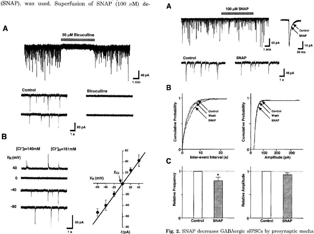
Fig. 1. GABAergic sIPSCs recorded from mechanically dissociated A1 neurons. (A) A representative trace of sIPSCs recorded before, during, and after the application of 50 \mu M bicuculline at a V_H of -60 mV. The external solution contained 300 nM TTX, 3 \mu M CNQX and 10 \mu M AP5. Insets represent typical traces with an expanded time scale. (B) Traces of sIPSCs recorded at V_H of -60, -40, 0, and +40 mV. Intracellular and extracellular Cl - concentrations were 140 mM and 161 mM, respectively. I-V curve for the mean amplitude of sIPSCs recorded at various V_H s. Each point is the mean of four neurons.
