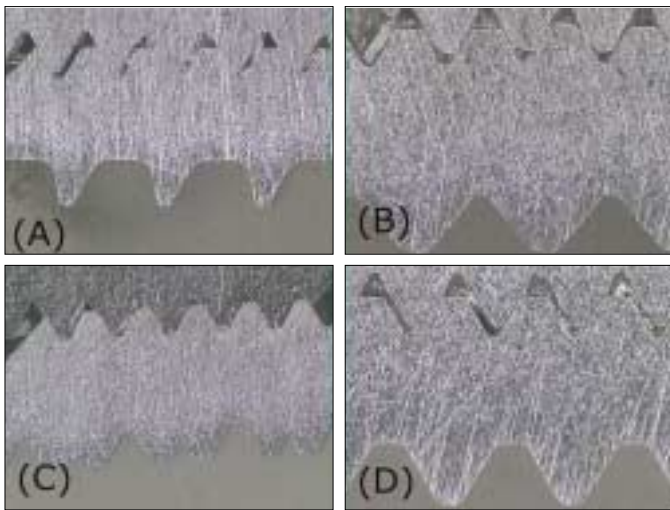
Fig. 6. Mechanical tolerance of various implants. A, Implantium (Dentium, Seoul, Korea); B, Astra (Astratech, Mölndal, Sweden); C, GS (Osstem, Pusan, Korea); D, M implant (Shinhung, Seoul, Korea).
