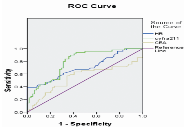
Figure 5. ROC Curve Analysis for Three Biological Markers. CYFRA21-1 and hemoglobin showed better predictive performance for OS than CEA (AUC= 0.791, 0.704, 0.545; P=0.000,0.000,0.409)
