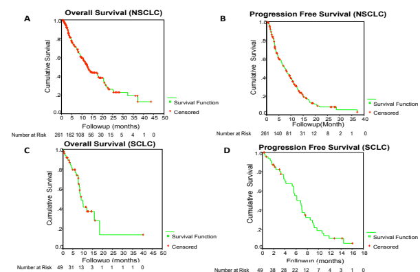
Figure 1. Kaplan Meir Survival Curves. A) Overall Survival, NSCLC, B) Progression Free Survival, NSCLC, C) Overall Survival, SCLC and D) Progression Free Survival, SCLC
