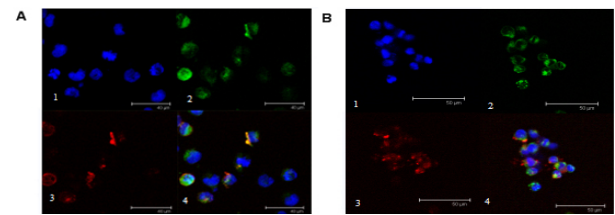
Figure 4. Co-localization of GalNAc-Ts in K562 Cell by Confocal Laser Scanning Microscopy. A: Control B: Group 2(1: DAPI stained nuclei, 2: PDIA4 labeled ER, 3: Lectin VVA and Tn antigen conjugate, 4: Merge of 1-3)
