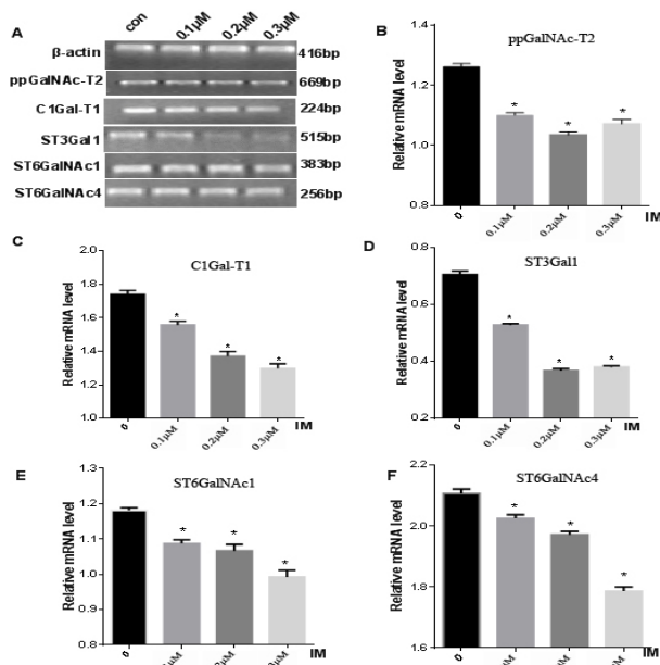
Figure 2. mRNA Expression Level of TACA Associated Glycosyltransferases on O-glycan. A: Control, Imatinib concentration: 0.1 μM, 0.2 μM, 0.3 μM; B-F: ppGalNAc-T2, C1Gal-T1, ST3Gal1, ST6GalNAc1 and ST6GalNAc4 mRNA expression level
