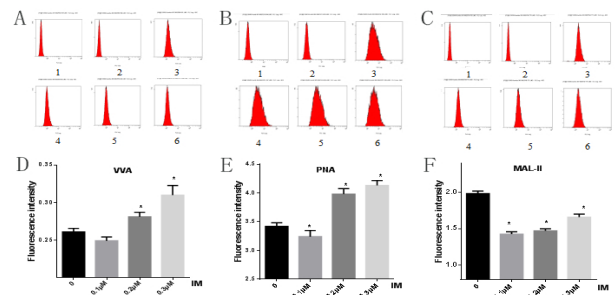
Figure 3. Changes of Tn, T and Sialyl-T Antigen Expression in K562 Cells after Imatinib Treatment.
