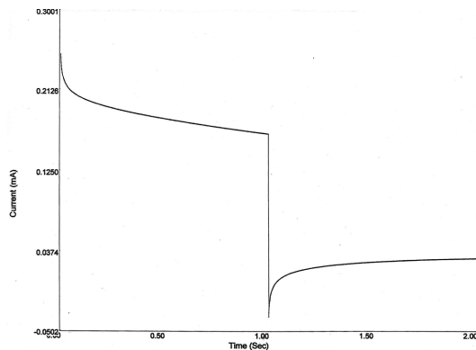
Fig. 7. Current transient resulting from the double step technique. Start potential: 0 (mV); first step E : -350 (mV); second step E: 0 (mV). [NaCl]: 0.002 M.
