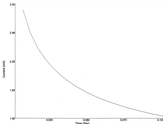
Fig. 6. Time profile of the double-layer charging current for a potential step in the electrolytic solution (0.1 M NaCl). Start potential : 0 (mV); step potential : -350 (mV).
