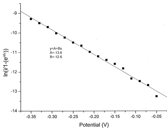
Fig. 3. Wave slope plot for the reduction of 2.0 \times 10^{-2} \text{ M} \text{H}_2\text{O}_2 in 0.1 \text{ M} \text{NaCl} .
