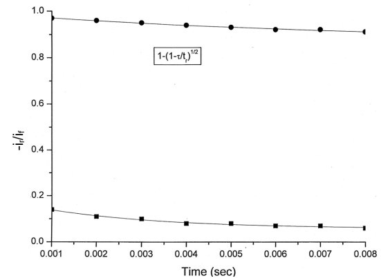
Fig. 8. Working curve for -i_r/i_s elicited from Fig. 7.
