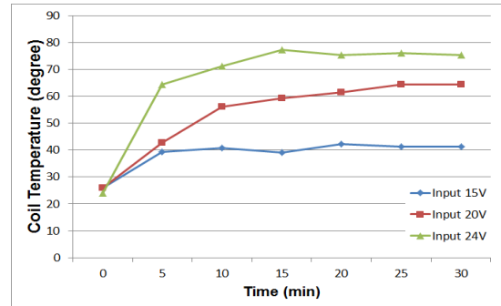
Fig. 11. Coil temperature
