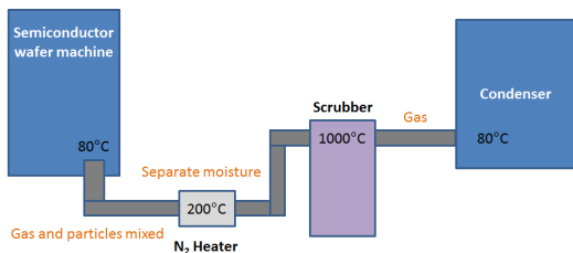
Fig. 1. Semiconductor wafer exhaust gas cleaning system.
