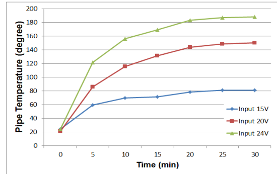
Fig. 10. Pipe temperature
