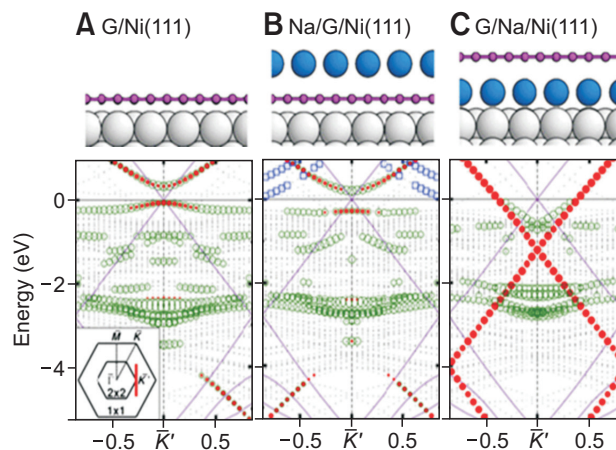
Fig. 2. Majority-spin band structures of graphene/Ni(111) (A), Na/graphene/Ni(111) (B), and graphene/Na/Ni(111) (C). The filled red (open green) circles represent C-derived (Ni-derived) surface states that contain more than 20% (40%) of charge in the graphene layer (topmost Ni layer).
