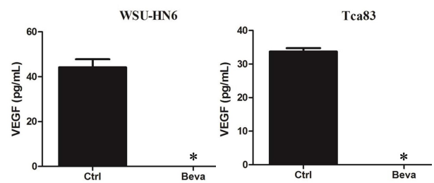
Figure 5. Bevacizumab Completely Neutralized Vascular Endothelial Growth Factor (VEGF) Secreted By Cancer Cells. Cells were treated with 100 \mu\text{g}/\text{mL} bevacizumab for 24 h following pretreatment with or without S3I-201, the specific STAT3 pathway inhibitor for 1 h. An ELISA was used to analyze the secreted protein collected from the supernatant. Results showed that secreted VEGF markedly decreased after bevacizumab treatment
