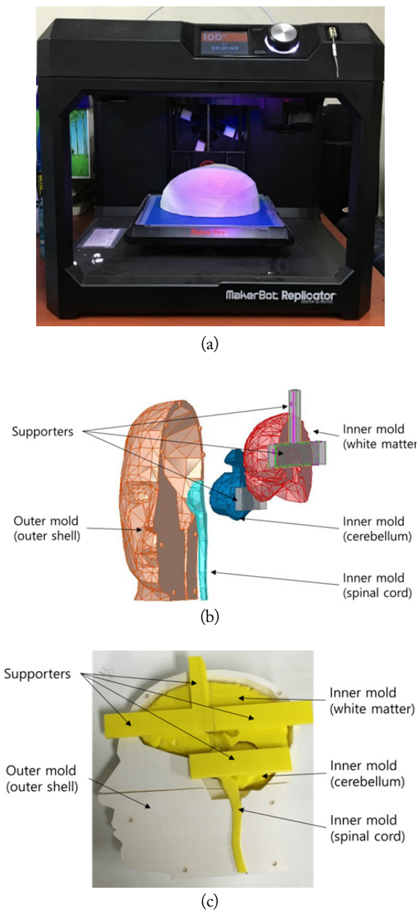
Fig. 1. The 3D printed molds for the phantom: (a) 3D printer, (b) 3D CAD data of the molds, and (c) photo of the molds.
