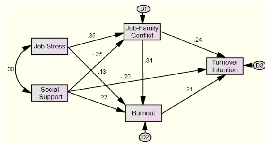
Fig. 2. Path analysis for the model with parameter estimates
