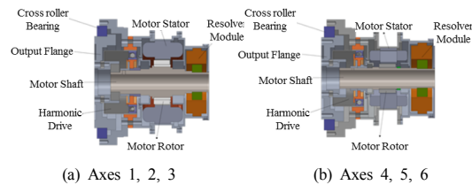
Fig. 7. Cross-section of developed motor
