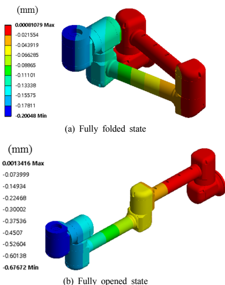
Fig. 12. Deformation results of robot arms under 5kgf load
