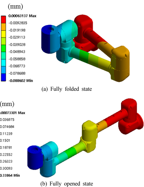
Fig. 11. Deformation results of robot arms under their self-weight
