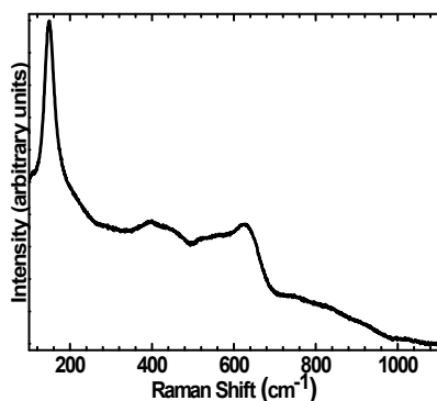
Fig. 4 Raman spectrum of oxide nanolayer on Ti-15Zr-5Nb alloy surface.
