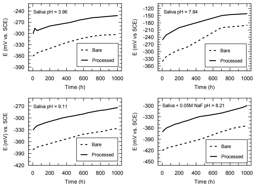
Fig. 9 Monitoring of the open circuit potential for bare and electrochemical processed Ti-15Zr-5Nb alloy in Carter-Brugirard saliva of different pH values, at 37 °C.
