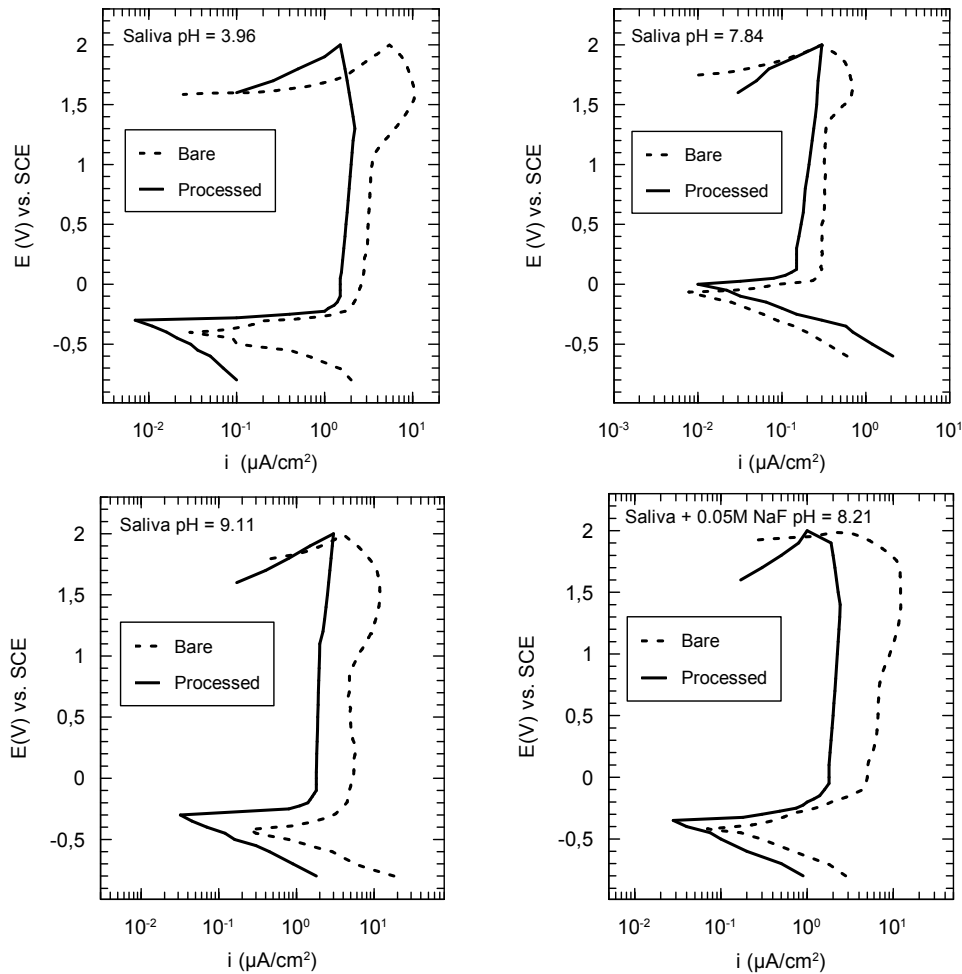
Fig. 5 Potentiodynamic polarisation curves for bare and electrochemically processed Ti-15Zr-5Nb alloy in Carter-Brugirard saliva of different pH values, at 37 °C.
