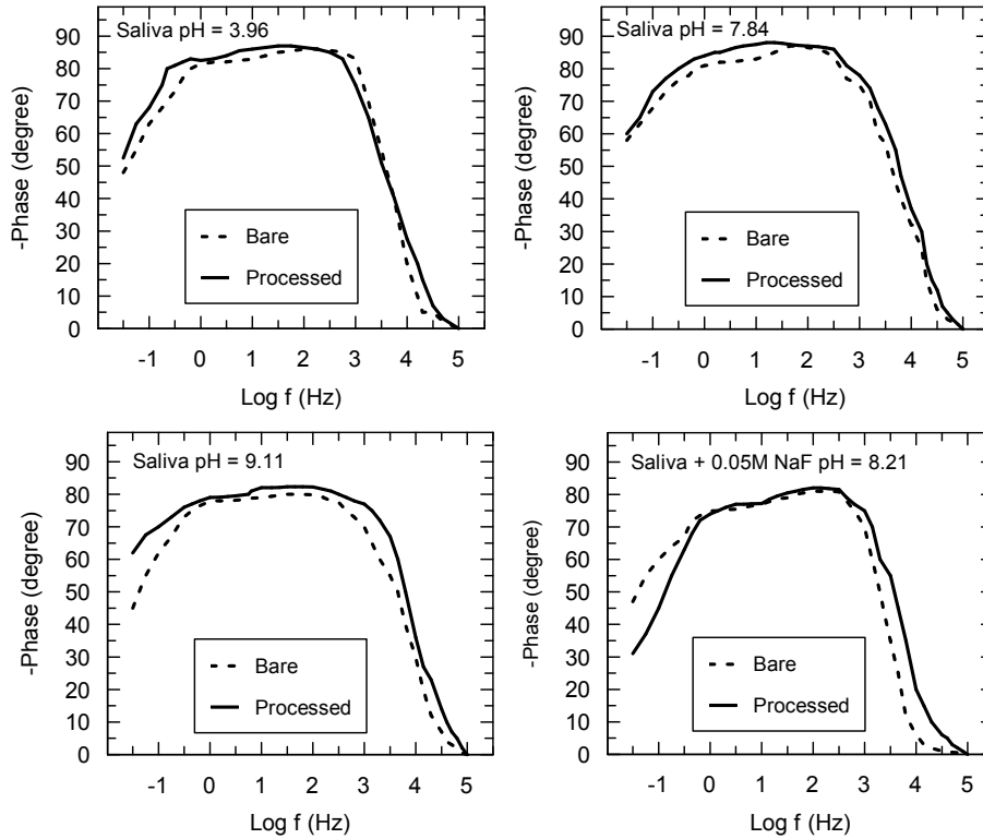
Fig. 7 Bode spectra for bare and electrochemical processed Ti-15Zr-5Nb alloy in Carter-Brugirard saliva of different pH values, at 37 °C.
