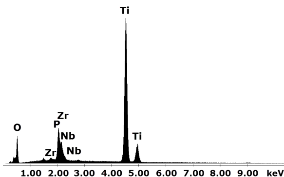
Fig. 3 EDS spectrum of oxide nanolayer on Ti-15Zr-5Nb alloy surface.
