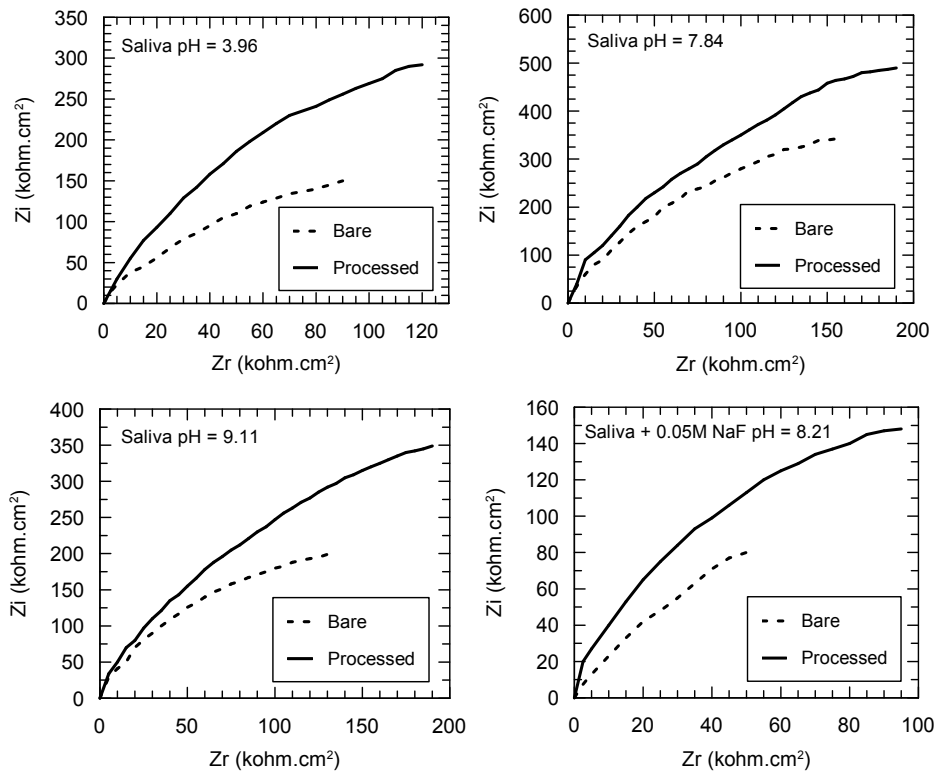
Fig. 6 Nyquist spectra for bare and electrochemical processed Ti-15Zr-5Nb alloy in Carter-Brugirard saliva of different pH values, at 37 °C.
