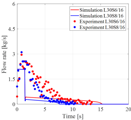
Fig. 10. Simulation and experimental results of the flow rate
