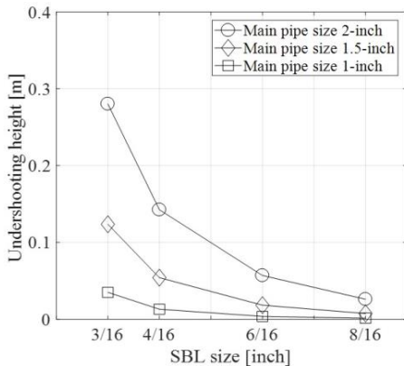
Fig. 2. UH results according to SBL sizes and main pipe sizes
