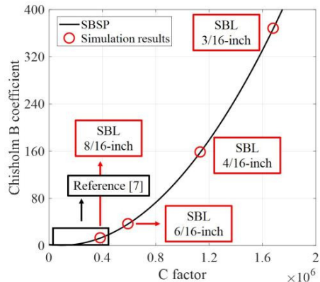
Fig. 3. Simulation results of C factor-Chisholm B coefficient according to SBL sizes
