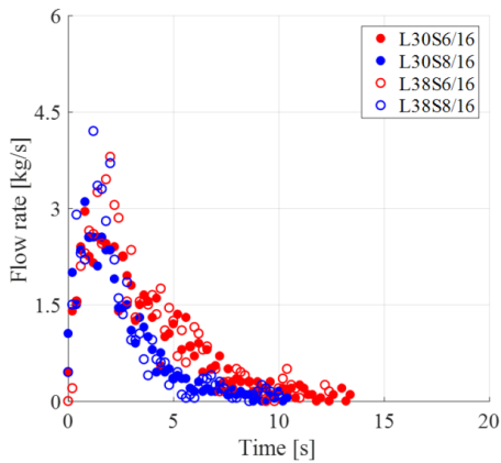
Fig. 8. The experimental results of the flow rate
