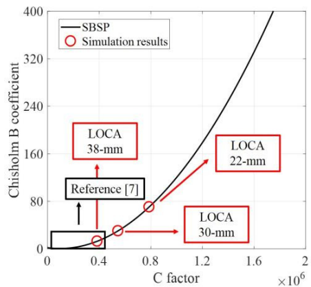
Fig. 5. Simulation results of C factor-Chisholm B coefficient according to LOCA sizes
