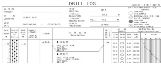
Fig. 3. Drill log[9]
