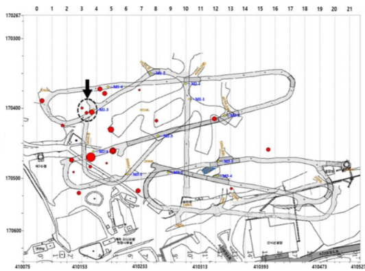
Fig. 5. Underground map[8]
