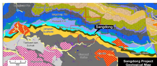
Fig. 2. Geological map[8]
