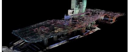
Fig. 10. Pointcloud by static scanner
