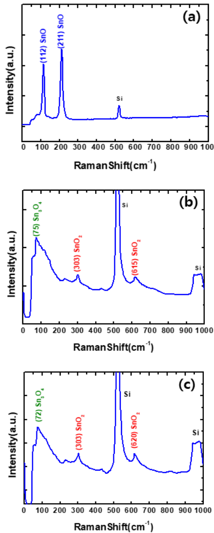
Fig. 3. Raman spectrum of as grown SnO (a), post-annealed SnO at 830 °C (b), and 1030 °C (c) respectively. (a) exhibits the SnO phase. SnO shows its inherent peak near 112 \text{cm}^{-1} and 211 \text{cm}^{-1} . SnO peaks show very high intensity due to their thick thickness and density. (b) & (c) exhibit the \text{SnO}_2 phase and \text{Sn}_3\text{O}_4 phase. As we can see, there're no more peak near 112 \text{cm}^{-1} and 211 \text{cm}^{-1} which means SnO phase has been removed by post annealing of SnO nanostructures. (b) shows the effect of post-annealing at 830 °C which shows various phase of tin oxide such as \text{Sn}_3\text{O}_4 and \text{SnO}_2 . Also we can observe that (c) has similar Raman spectrum compare to (b) which means \text{Sn}_3\text{O}_4 appear during oxidation process of SnO in oxygen atmosphere.
