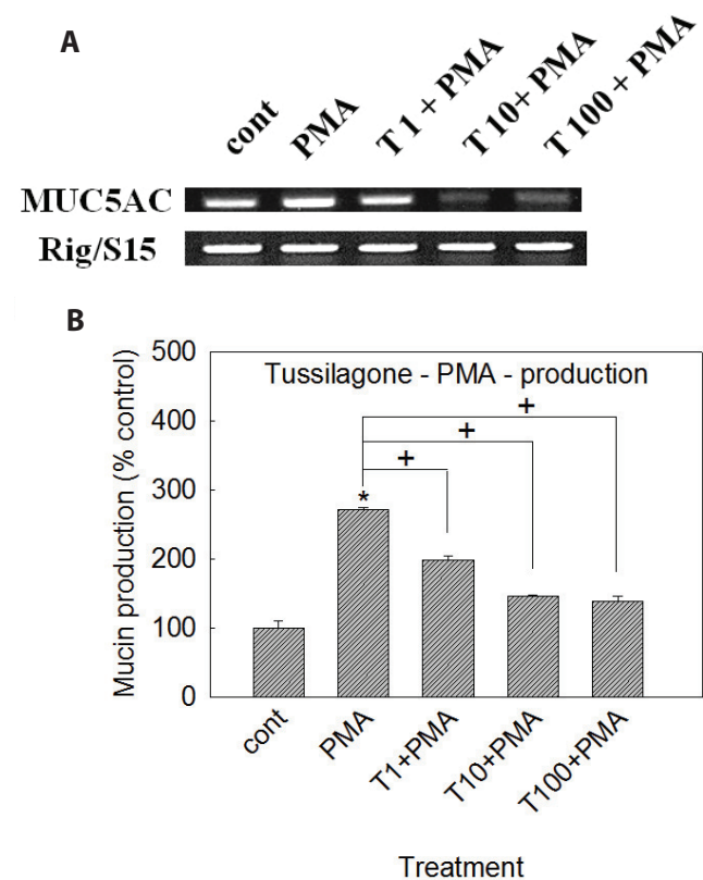
Fig. 3. Effect of tussilagone on PMA-induced MUC5AC mucin production and gene expression from NCI-H292 cells. NCI-H292 cells were pretreated with varying concentrations of tussilagone for 30 min and then stimulated with PMA (10 ng/ml) for 24 h. Cell lysates were collected for measurement of MUC5AC mucin production by ELISA. Each bar represents a mean±S.E.M. of 3 culture wells in comparison with that of control set at 100% (B). MUC5AC gene expression was measured by RT-PCR (A). Three independent experiments were performed and the representative data were shown. *significantly different from control ( p<0.05 ). †significantly different from PMA alone ( p<0.05 ). cont: control, T: tussilagone, concentration unit is μM.
