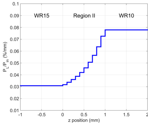
Fig. 5. Conductor loss of TE_{10} in the linearly tapered rectangular waveguide.
