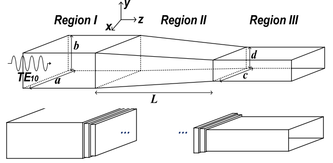
Fig. 1. Rectangular waveguide transition structure: a tapered rectangular waveguide.
