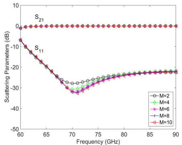
Fig. 2. Convergence test for the number of sub-waveguides.
