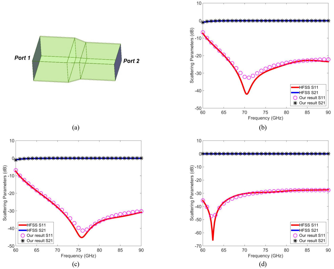
Fig. 3. (a) Simulation model of the tapered rectangular waveguide in ANSYS HFSS and a comparison of our computation results with the HFSS simulation results. (b) V to W, (c) E to W, and (d) V to E transitions.
