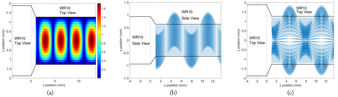
Fig. 4. (a) Electric field distribution at the center of the receiving waveguide and (b) side view and (c) top view of surface current density on the walls of the receiving waveguide.
