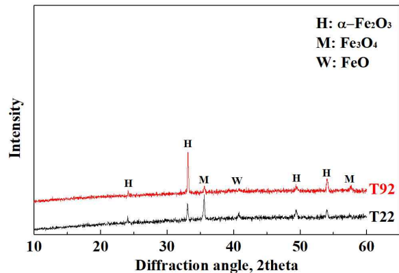
Fig. 4 XRD patterns of the oxide film on T22 and T92 steel in 6O 2 -16CO 2 -2SO 2 gas at 650 °C for 500 h.
