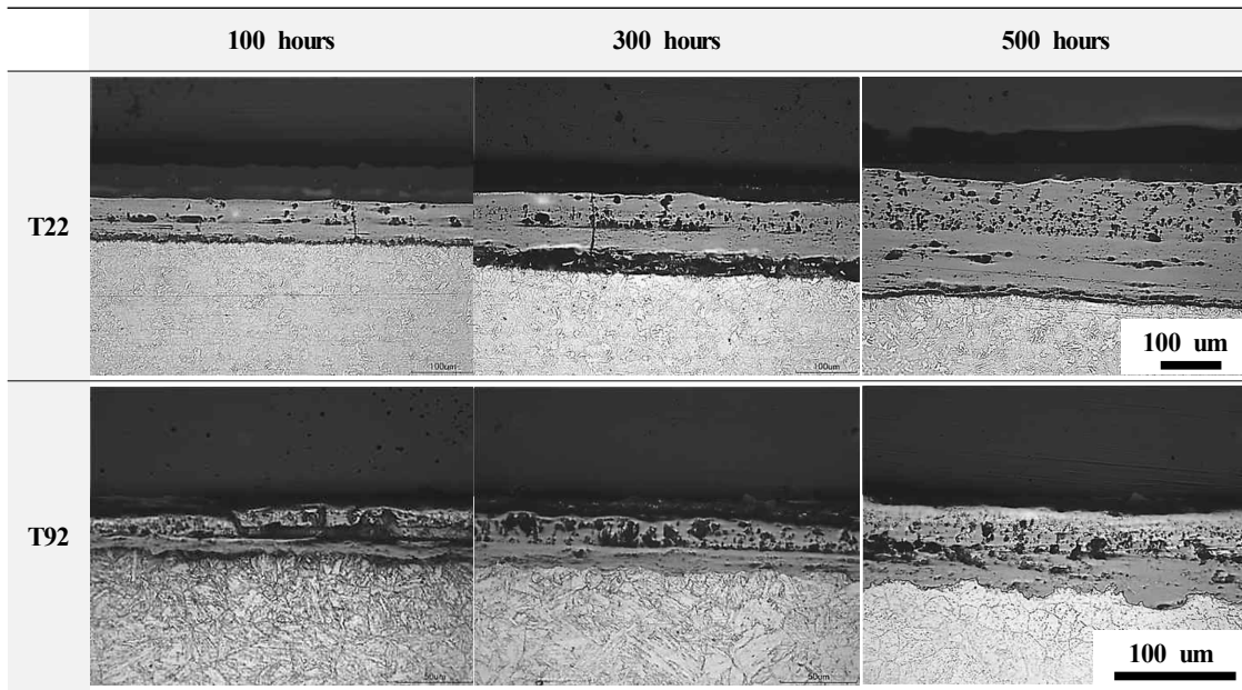
Fig. 2 Cross-sectional OM images of T22 and T92 steel 6O 2 -16CO 2 -2SO 2 gas at 650 °C with time.
