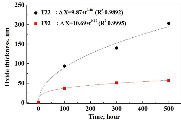
Fig. 3 Thickness of oxide film for T22 and T92 steel with time in 6O 2 -16CO 2 -2SO 2 gas at 650 °C.
