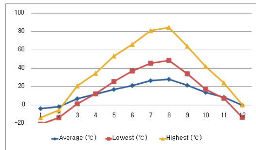
Fig. 1. Monthly temperature in Incheon (2018)
