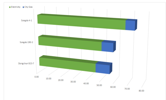
Fig. 5. Energy consumption divide by Floor Area
