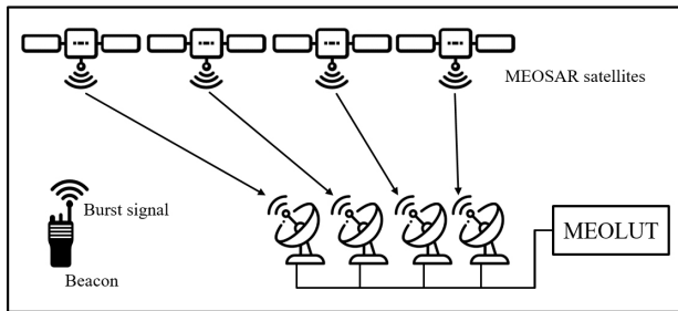
Fig. 2. MEOLUT system with directional dish antenna.
