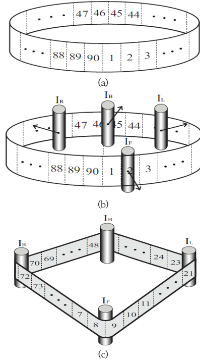
Fig. 3. Calculating I_F, I_B, I_L, I_R with calibration.
