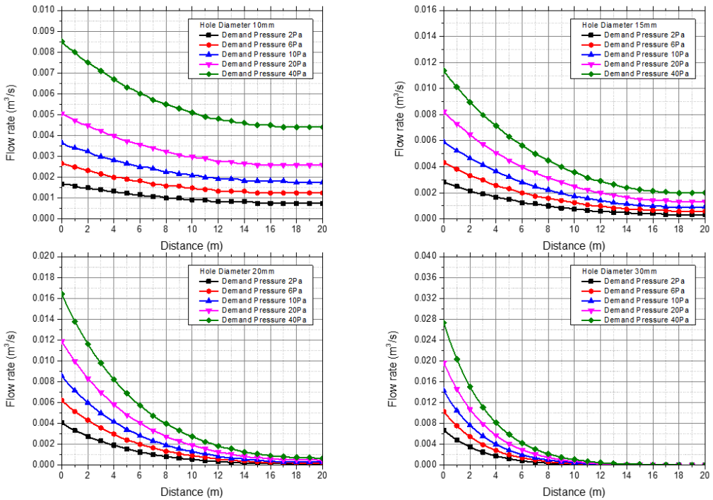
Fig. 3. Flow rate distribution of ventilation hole.
