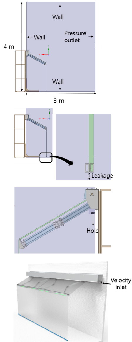
Fig. 1. Geometry and boundary condition.
