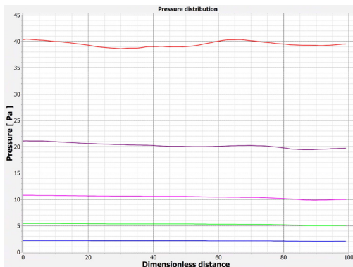
Fig. 4. Pressure distribution at center line of fire safety curtain.
