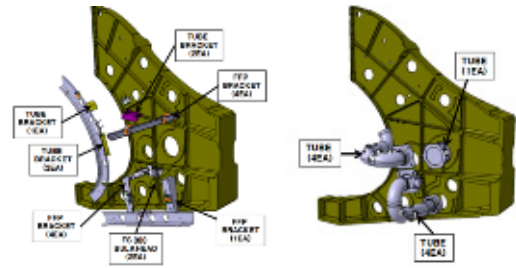
Fig. 10. Strain Gage Install Location
