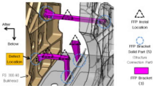
Fig. 3. Install Configuration of FFP
