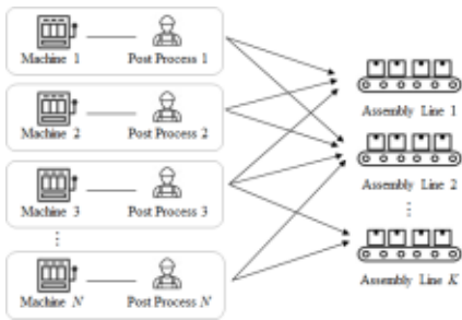
Fig. 1. Manufacturing system structure assumed in this study
