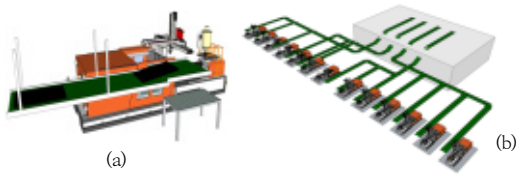
Fig. 4. Conveyor System (a) Conveyor for transporting injections (b) Overall structure of conveyor system
