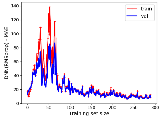
Fig. 5. Learning curves on the training set and validation set as a function of the training set size; DNN (optimizer=RMSprop) and M setup.
