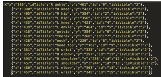
Fig. 3. PoseNet Key Points Extraction example
