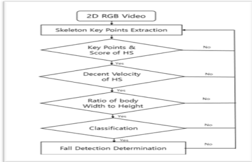
Fig. 1. Architecture of FDHG
