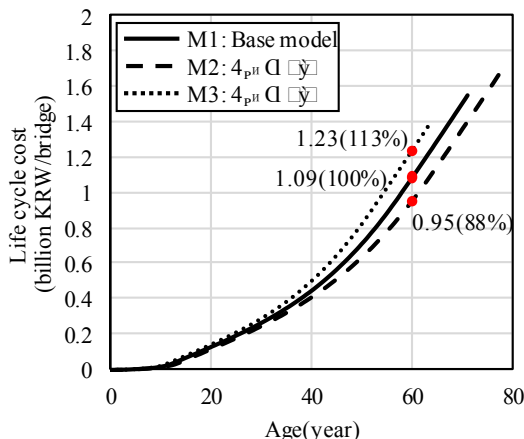
Fig. 8. Life cycle cost according to service life
