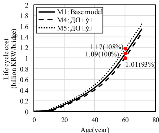
Fig. 9. Life cycle cost according to deterioration rate
