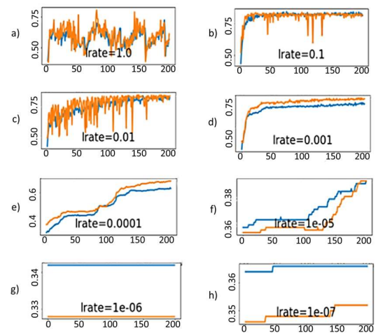
Fig. 9: the effect of different Learning Rates. a) too large lrate result in failure to learn, b) lrate 0.1 result in ability to learn, c) lrate 0.01 has showed good result, d) lrate 0.001 results in strong model performance on train and test set, e) lrate 0.0001 poor performance, g) and h) too small lrate result in inability to learn.
