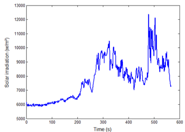
Fig. 9 Global solar radiation intensity
