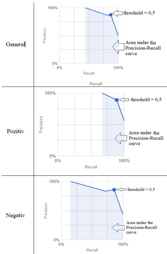
Fig. 5 Precision-Recall curves.
