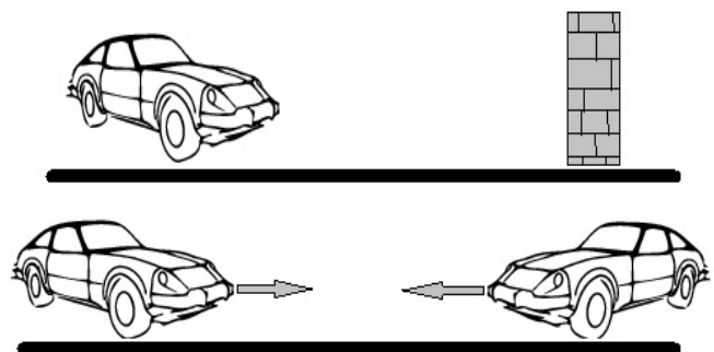
Figure 2. Probability_of_Collision_Occurrence
